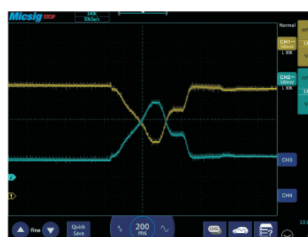
Throttle Position
