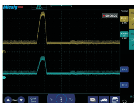
Accelerator Pedal
