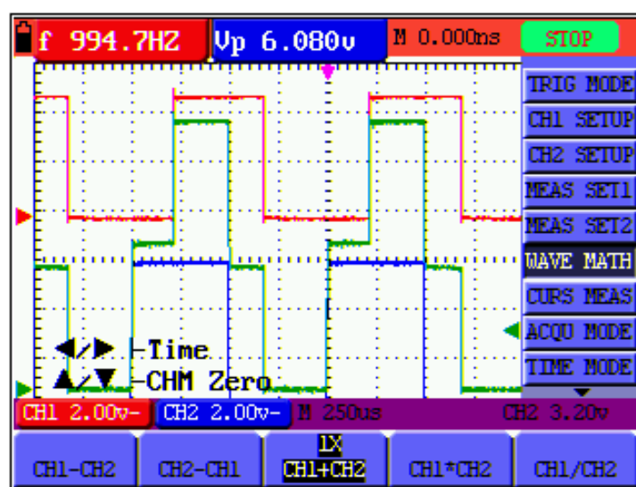
figure 37: Waveform Mathematics
