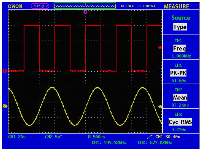
Fig.69 Automatic Measurement
