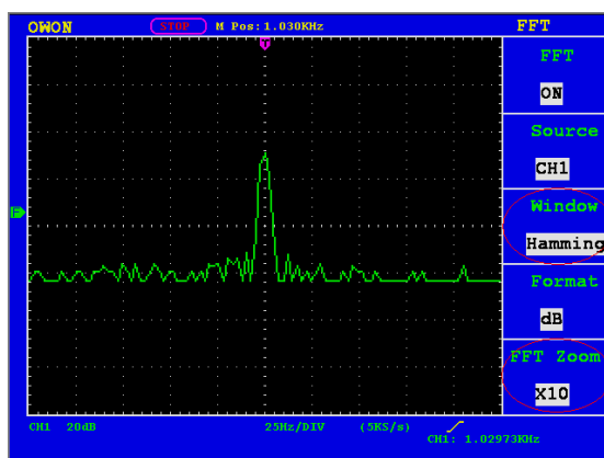
Fig.29. Hamming window
