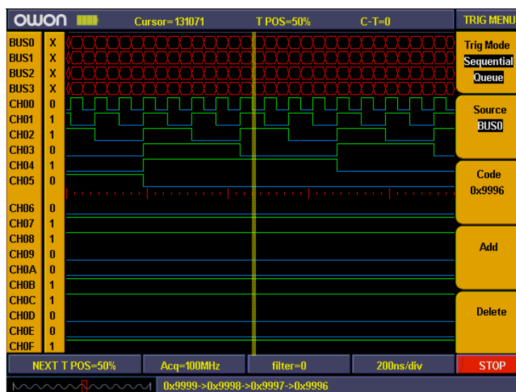
Fig. 87: Sequential queue trigger
