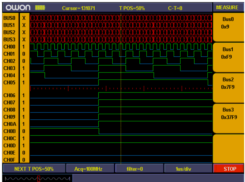
Fig.98: Bus measurement
