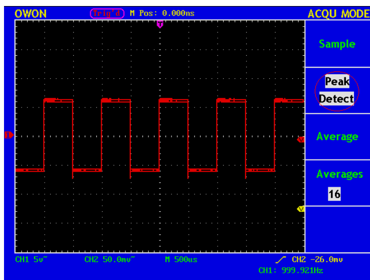
Fig. 111 Wave Form of the Signal Containing Noises
