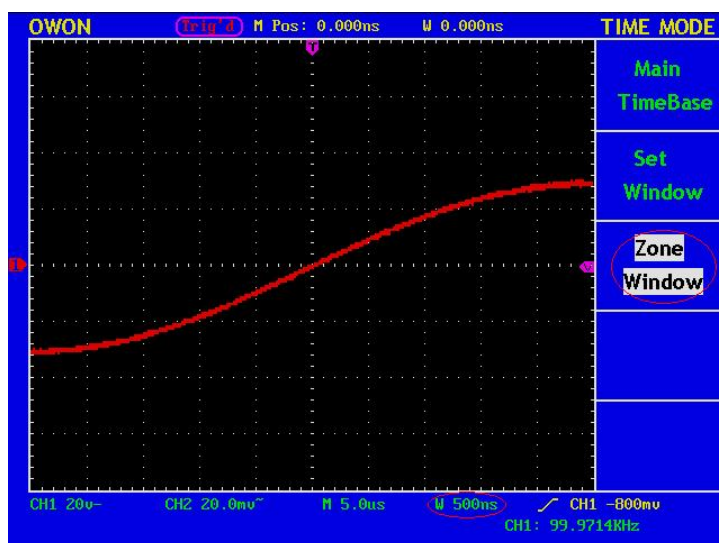
Fig. 37 Zone Window
