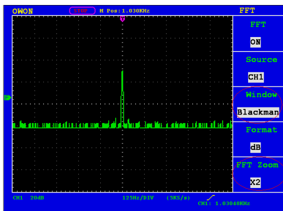
Fig.28. Blackman window
