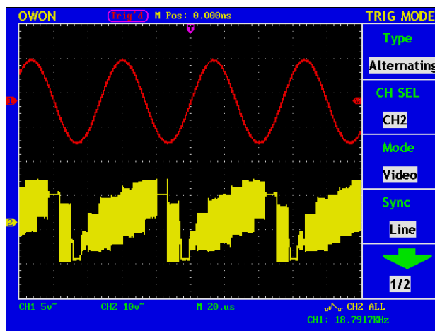
Fig. 51 Alternate trigger Oscillogram
