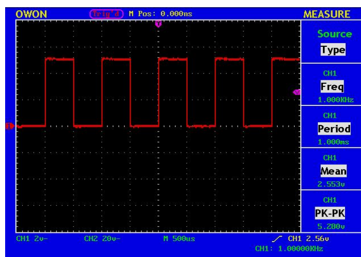
Fig. 108 Waveform of Automation Measurement
