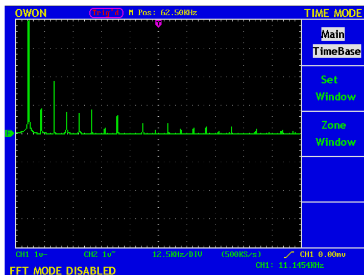
Fig.36 FFT mode disabled
