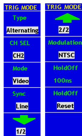
Fig.50: Alternate video trigger menu
