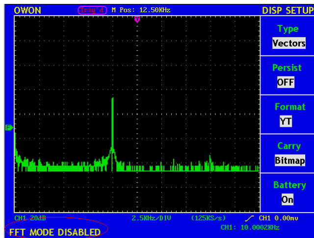
Fig.61 FFT mode XY Format Disable
