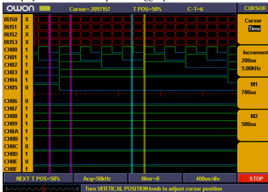
Fig. 106: Cursor time measurement
