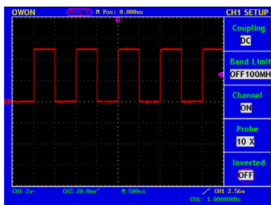
Fig. 25 Wave Form not inverted
