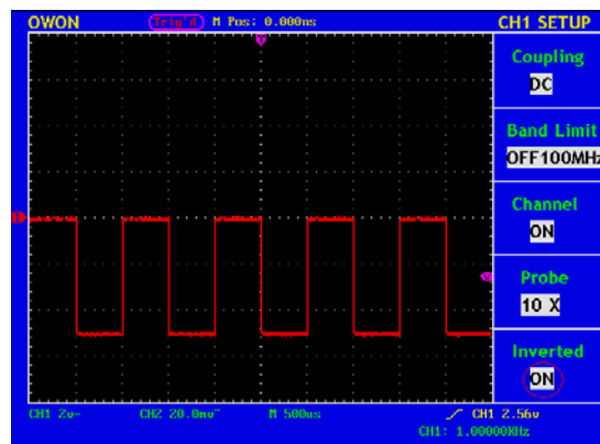
Fig. 26 Wave Form Inverted
