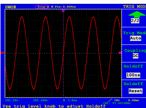
Fig. 46 Edge trigger (the second menu)
