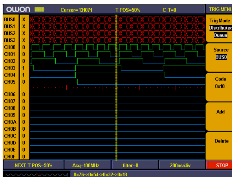
Fig.89: Distributed queue trigger
