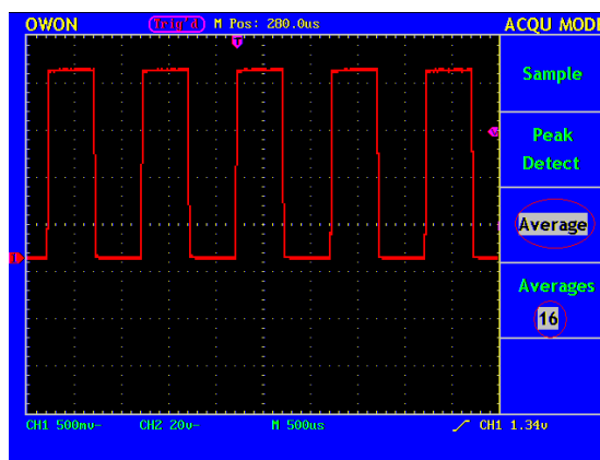
Fig. 55 Average on with reduced noise on waveform
