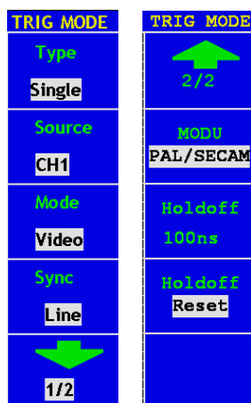
Fig. 47 Video trigger menu
