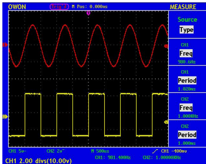
Fig. 32 Information about Vertical Position
