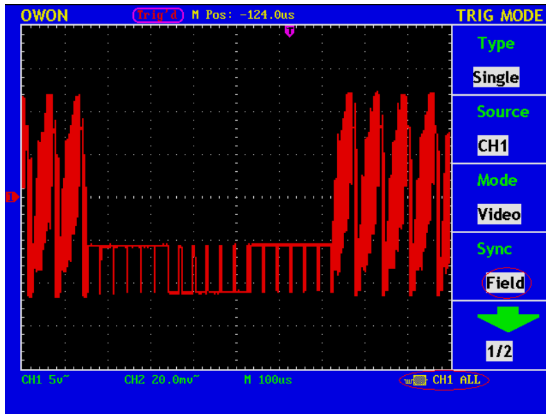
Fig. 114 Wave Form Obtained from Video Field Trigger
