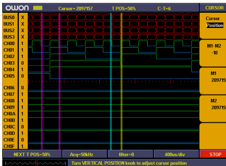
Fig.107: Cursor position measurement
