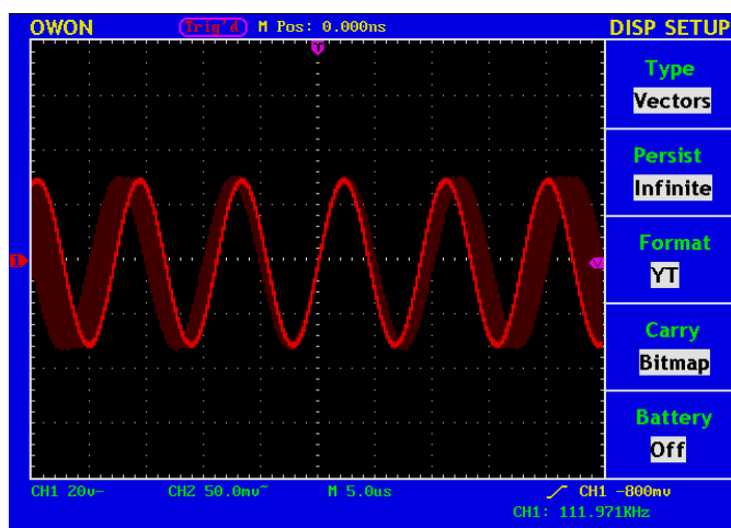
Fig. 59 Infinite Persistence Display
