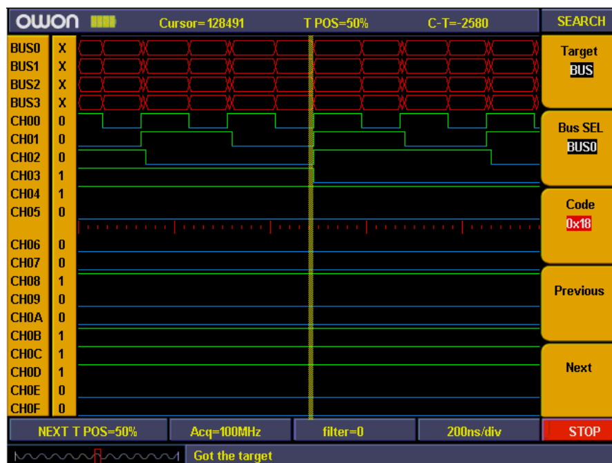
Fig.102: Search Bus
