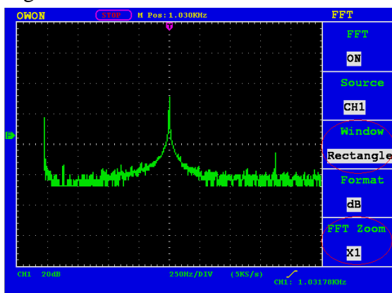
Fig.30. Rectangle window
