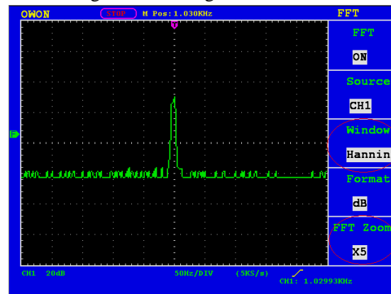
Fig.31. Hanning window
