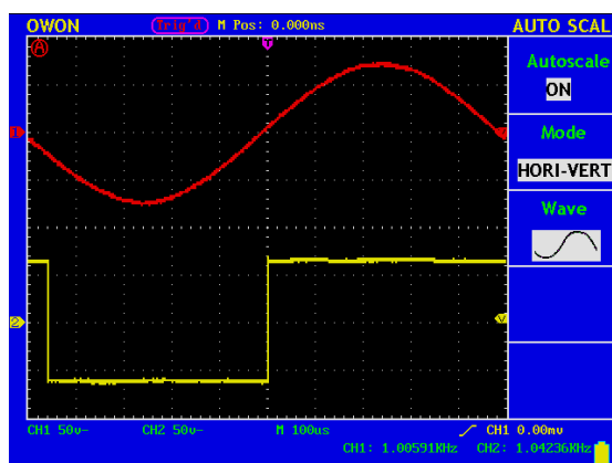
Fig.77 single cycle mode
