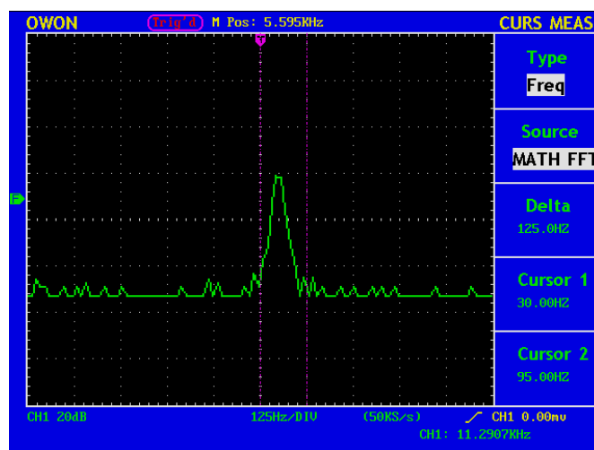
Fig.75 wave of Freq cursor measurement
