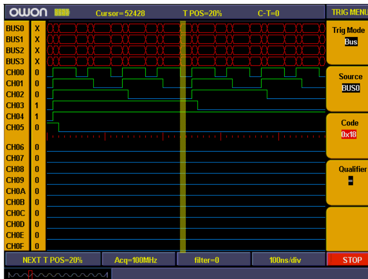
Fig.83: Bus trigger
